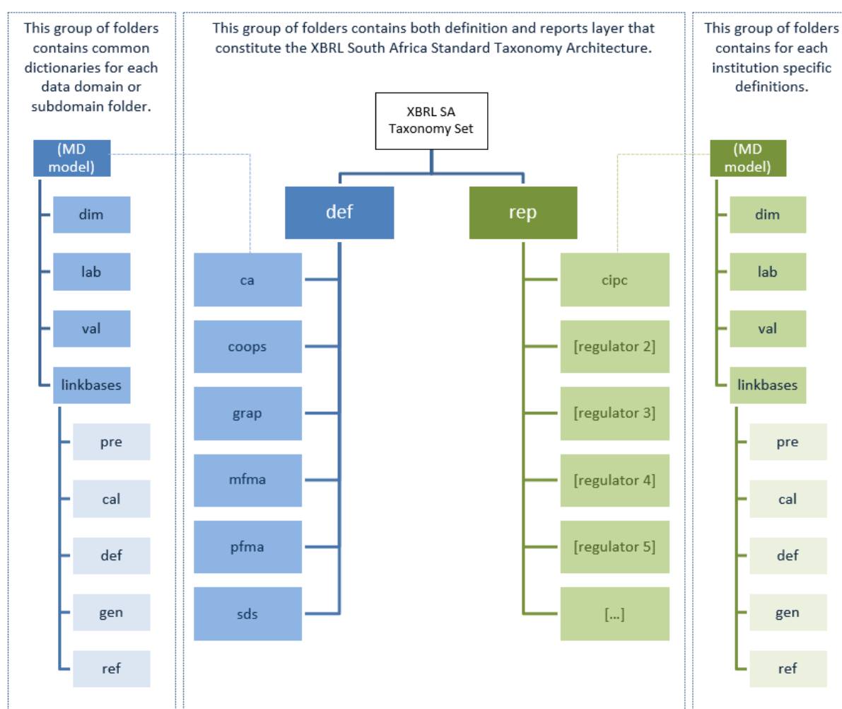
Figure 2: High-level physical modularization of the CIPC XBRL Taxonomy
